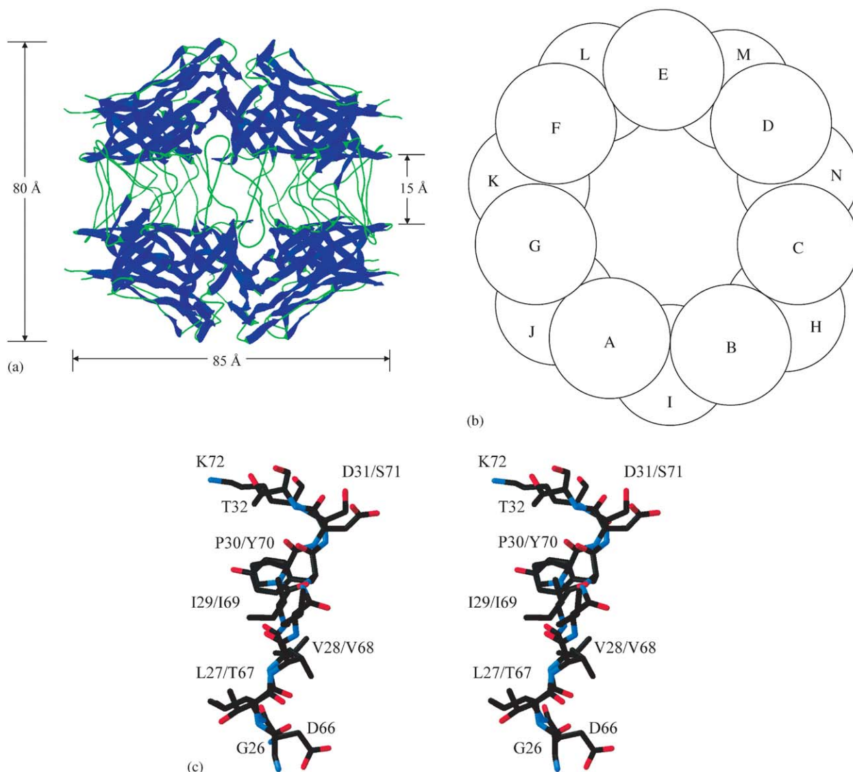
Fig. 3 The Mtcnp10 tetradecamer. (a) Viewed along 2-fold NCS axis. (b) Sketch of the staggered arrangement of subunits viewed down the seven-fold NCS axis. (c) Superposition of polypeptide segments 26–32 and 66–72 of subunit K associated with bone resorption activity. This figure was prepared using SwissPdbViewer .
