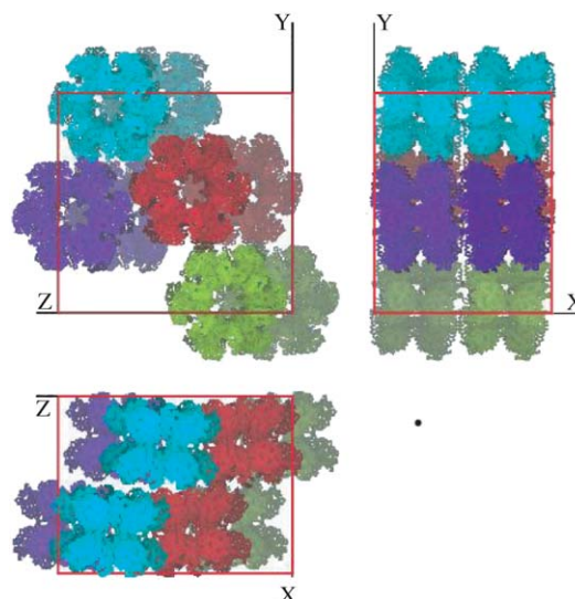
Fig. 4 Three-dimensional structure of M. tuberculosis glutamine synthetase. The figure shows the crystal packing of M. tuberculosis GS molecules in the P2_12_12_1 crystal form. Three orthogonal views of the unit cell are illustrated. The action of the four symmetry operators are represented by different colors. Two dodecamers of identical color comprise one asymmetric unit.
