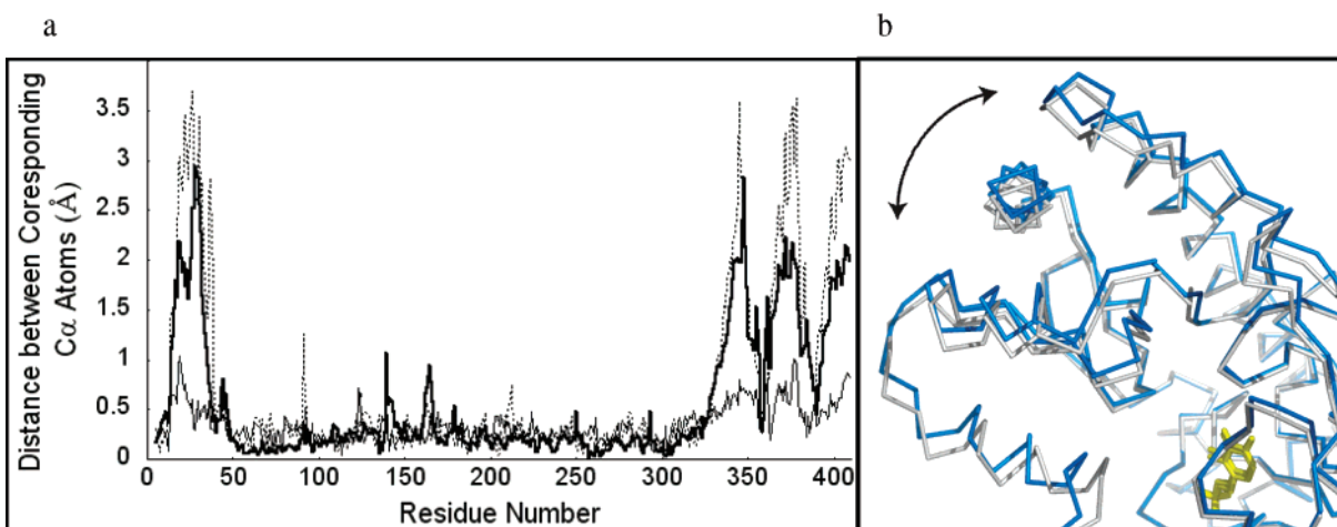
FIGURE 3: Small domain (residues 16–47 and 326–409) movement accompanies complex formation. (a) The dotted line shows movement of C_{\alpha} atoms between the closed and half-open conformations of wild-type eAATase. The solid thin and thick lines show the distance between corresponding C_{\alpha} atoms of the unliganded and Hca complexes of HEX and HEX + A293D, respectively. Upon association of Hca, HEX remains closed while HEX + A293D adopts a new conformation intermediate between the closed and half-open states; there is significant movement of HEX + A293D C_{\alpha} atoms in the small domain that reach nearly 3 Å. (b) One of the small subunits of unliganded HEX (gray) and HEX + A293D (blue) with bound PLP (yellow). While the backbones of the large domains for both structures are almost exactly superimposable (not shown), those of the small domains are not.
