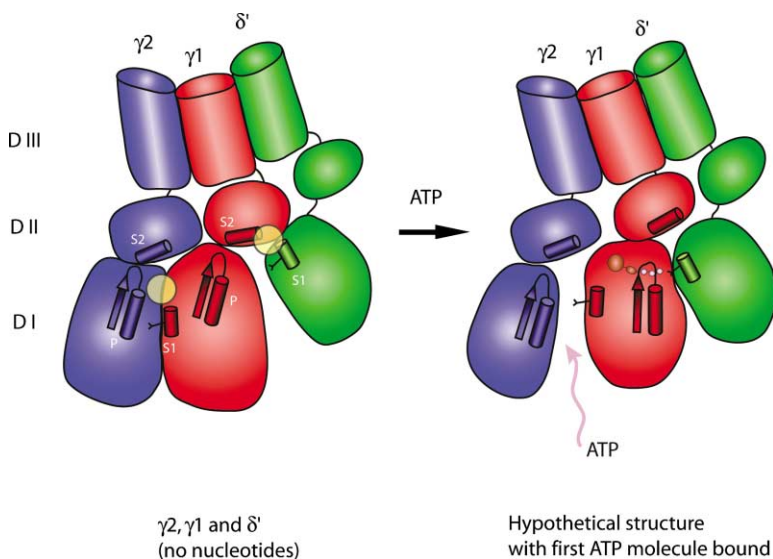
Figure 8. Schematic Diagram of Potential Rearrangement in the Clamp Loader Complex upon Nucleotide Binding
