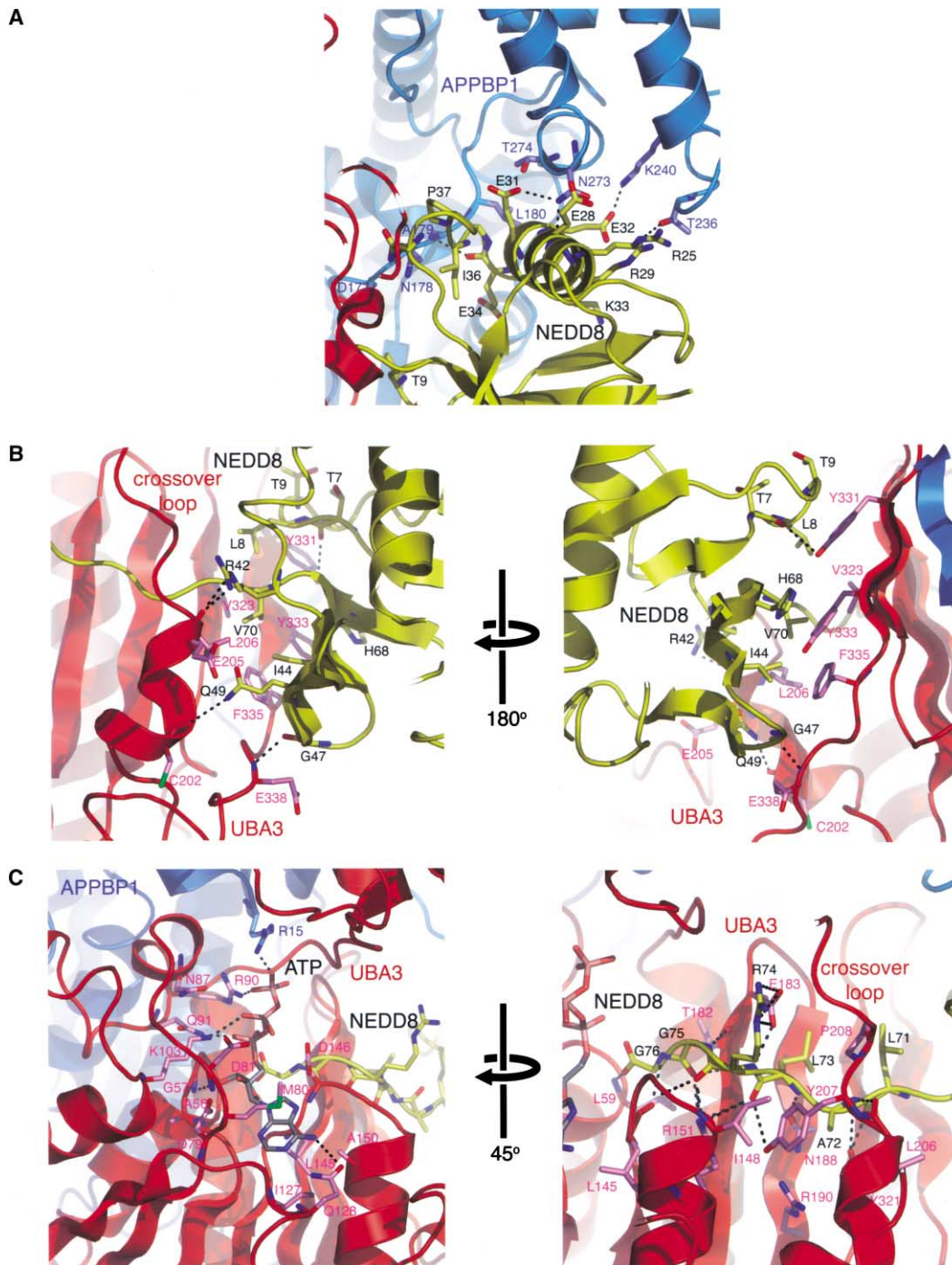
Figure 4. Detailed Views of NEDD8 and ATP Interactions with APPBP1-UBA3
