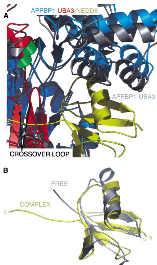
Figure 5. Conformational Changes in APPBP1-UBA3 and NEDD8 Accompanying Complex Formation
