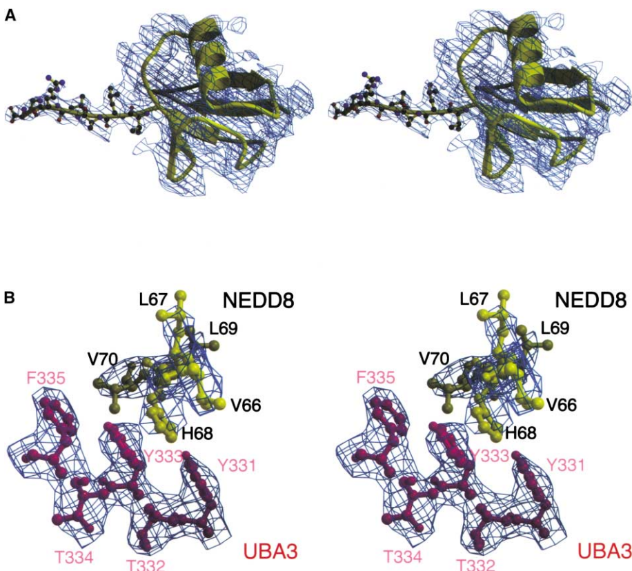
Figure 1. Stereo Views of Electron Density Maps
