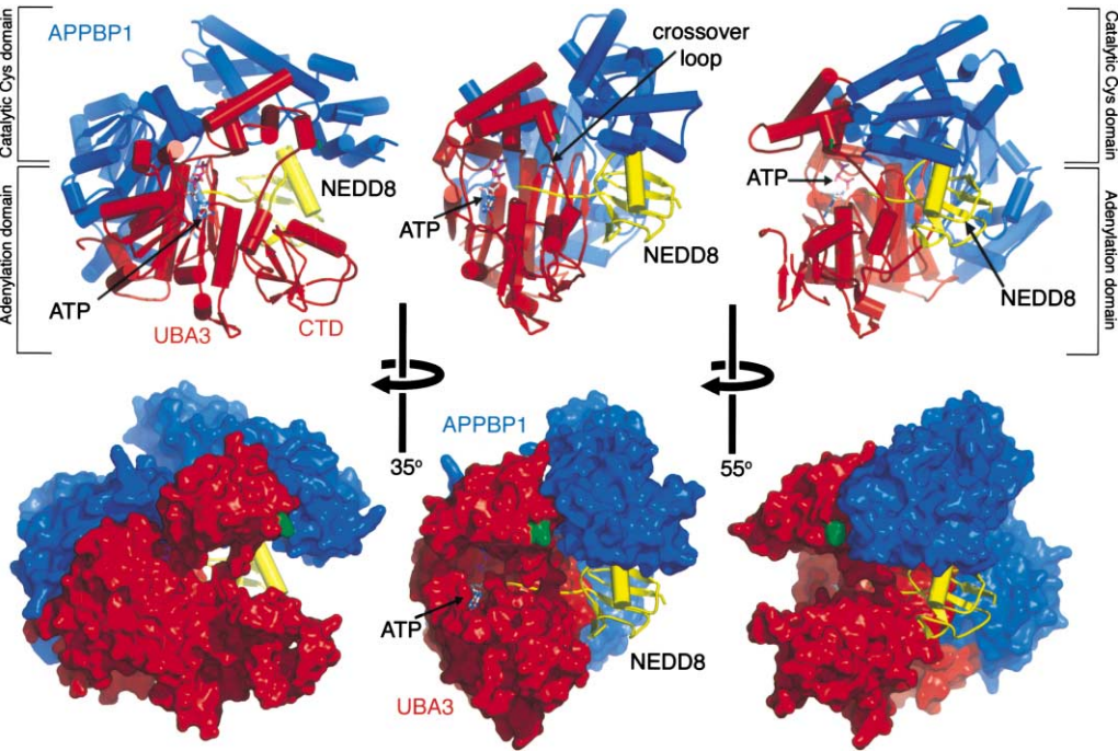
Figure 2. Overall Structure of the APPBP1-UBA3-NEDD8-ATP Complex Three views of the complex are shown in cartoon (top) and space-filling representations (bottom), each view a 35°–55° rotation around the y axis as indicated. APPBP1 is shown in blue, UBA3 in red, NEDD8 in yellow, and the position of the catalytic cysteine (C216A here) in green. The location of ATP is indicated in each view in the cartoon representations. The adenylation domain, the catalytic cysteine domain, and the C-terminal domain (CTD) are indicated. Figures were made using Pymol (DeLano, 2002).
