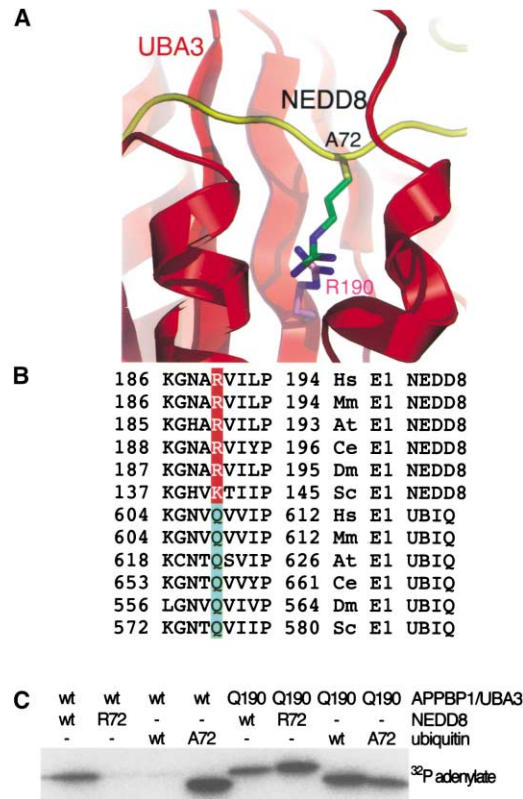
Figure 6. A Single Conserved Arginine in APPBP1-UBA3 Selects against Ubiquitin Activation
