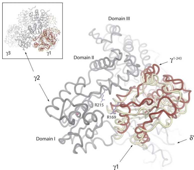
Figure 7. Potential Conformational Change at the \gamma 1 - \gamma 2 Interface Induced by Nucleotide Binding
