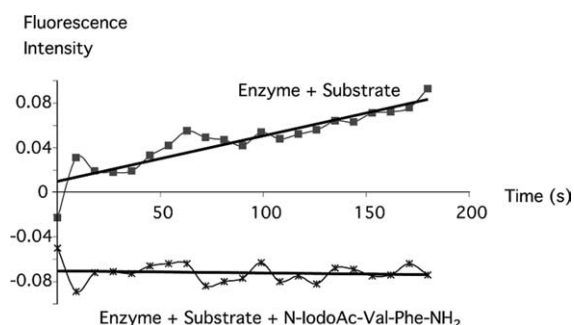
Figure 4. Assay of activity of redissolved crystals of HAV 3C protease C24S modified at the \epsilon 2-nitrogen of His102 by alkylation with N-Cbz-L-serine \beta -lactone (1a). The assay was done using fluorogenic peptide substrate Dabcyl-GLRTQSFS-Edans without inhibitor and also with addition of an excess of the irreversible inactivator, N-iodoacetyl-Val-Phe-amide.
