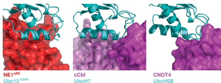
and Ubch5B are shown in cyan. The corresponding regions of the first turn of the N-terminal helix in Ubc12 core , Ubch7, and Ubch5B are labeled "α1," and are involved in binding to NE1 ulid , c-Cbl, and CNOT4, respectively.
