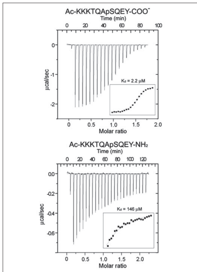
FIGURE 1. The MDC1 BRCT domain specifically recognizes the free carboxyl terminus of the \gamma -H2AX tail. Shown are sample ITC experiments showing titration of the MDC1 BRCT domain with the \gamma -H2AX peptide bearing a free carboxylate at the COOH terminus (top panel) or an amidated COOH terminus (bottom panel). The titration curves (insets) were used to determine the dissociation constants. The K_d values shown are the average of three independent experiments.
