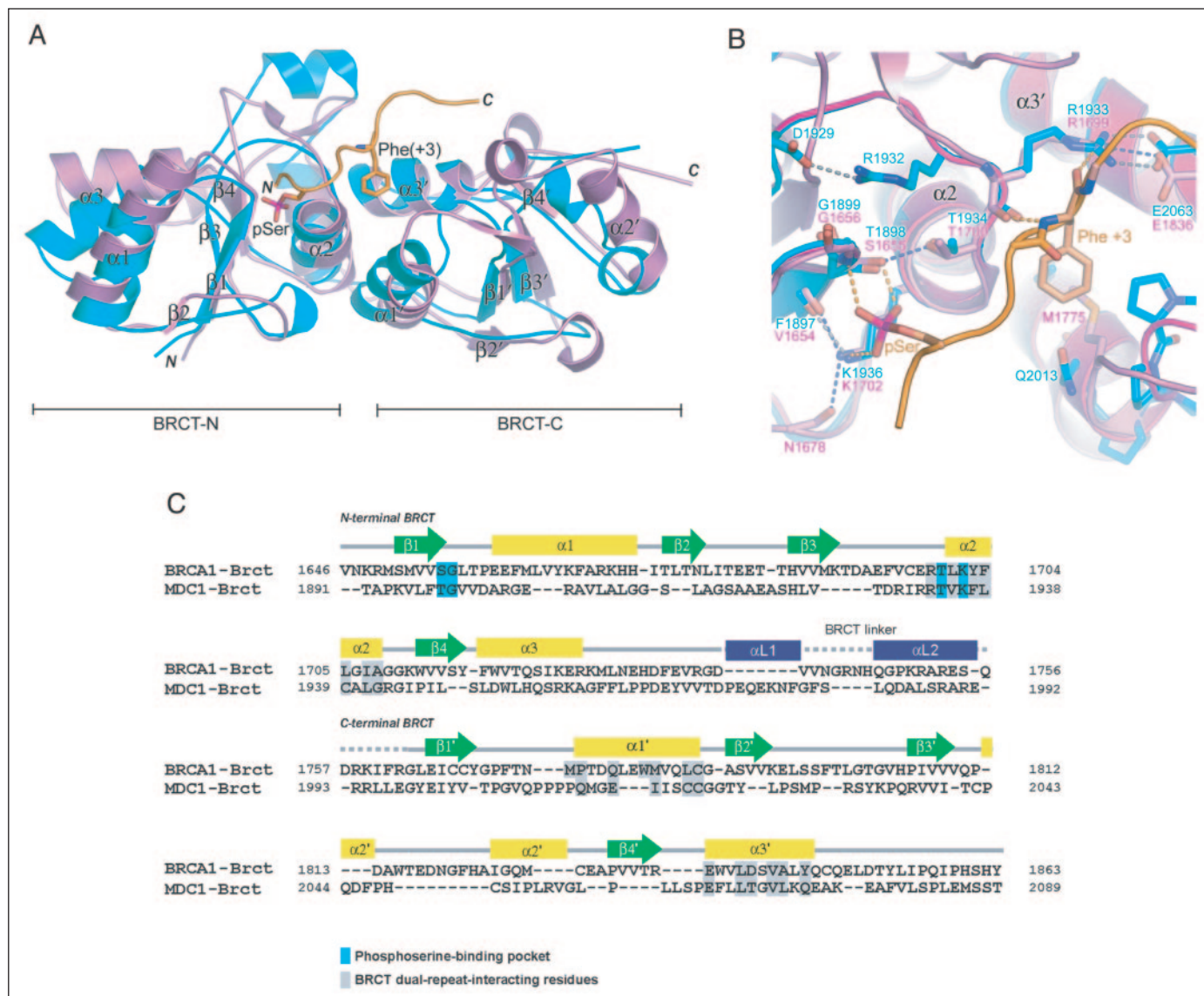
FIGURE 2. Structure of the tandem BRCT repeats of MDC1. A , overview of the MDC1 BRCT structure (cyan) aligned with the structure of the BRCA1 BRCT (magenta) bound to an optimized phospho-peptide target (orange) (Protein Data Bank accession code 1T2V). B , details of the phosphopeptide recognition surfaces of BRCA1 and MDC1, colored as in A . Residues involved in peptide binding are labeled and shown as sticks. C , sequence alignment of the MDC1 and BRCA1 BRCT repeats. The secondary structure of MDC1 is indicated, and residues conserved in the phosphoserine binding pocket are highlighted in blue. Residues involved in the head-to-tail packing of the NH 2 - and COOH-terminal BRCT repeats are shaded in gray.
