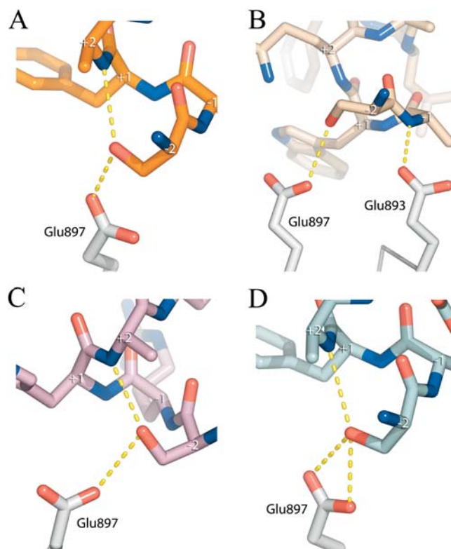
Figure 6. Interactions of Ser-2 with Glu897 Interactions between Ser-2 of the peptides (A) FxxLW, (B) WxxLF, (C) WxxVW, and (D) FxxFF and Glu897 of the LBD. Peptide alpha carbons are labeled. DOI: 10.1371/journal.pbio.0020274.g006
