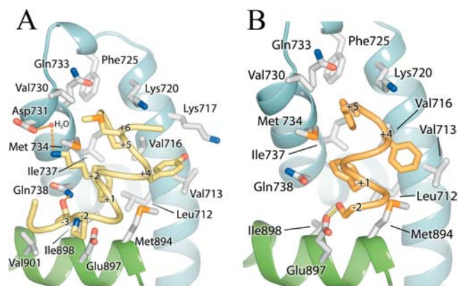
Figure 7. Interactions of FxxYF and FxxFF with the AR LBD FxxYF (A) and FxxFF (B) bound to the AR AF-2 interface. FxxYF and FxxFF are shown as yellow and orange C \alpha coils, respectively. The LBD is depicted as in Figure 3. DOI: 10.1371/journal.pbio.0020274.g007
