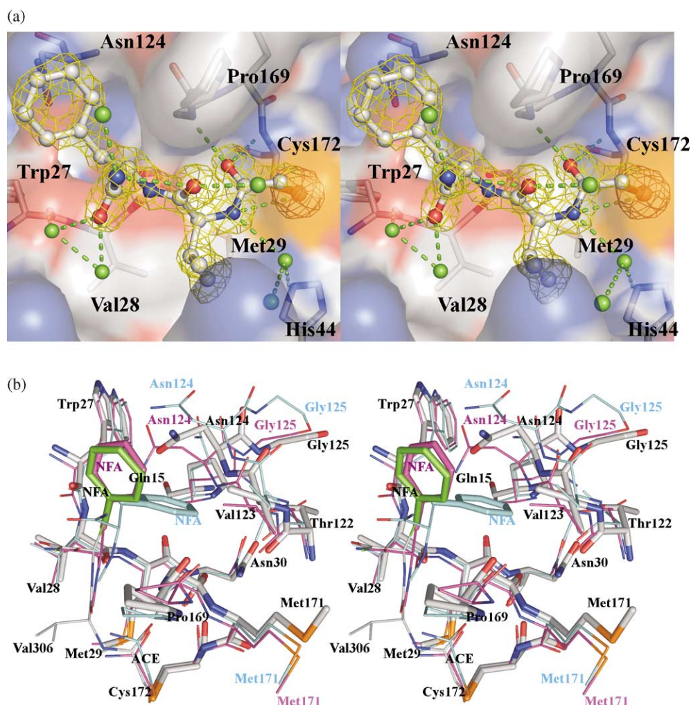
Figure 12. Interactions involving atoms of the IVF inhibitor in the active site of 2A4O. (a) The omit |F_o| - |F_c| electron density map contoured at 3 sigma level with the final refined model of the IVF (iodoacetyl-Val-NFA) superimposed. NFA refers to phenylalanine-amide. The density of the inhibitor is continuous from the 2|F_o| - |F_c| density of the sulfur atom in Cys172, indicating a covalent linkage. The IVF inhibitor is represented in ball and stick and colored similarly as in Figure 8. The residues forming hydrogen bonds or van der Waals interactions with IVF inhibitor are shown in sticks. Also shown are several water molecules in green that interact with the covalently bound inhibitor via hydrogen bonds. (b) A structural alignment of the IVF inhibitors and S2' sites in 2A4O and molecules A, B of the 1QA7 structure. The structures are distinguished by the coloring of carbon atoms: gray is for 2A4O, cyan for molecule A and magenta for molecule B. Residue labels (color codes same as carbon atoms) are provided where the three structures differ significantly.
