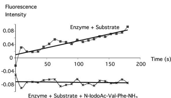
Figure 4. Assay of activity of redissolved crystals of HAV 3C protease C24S modified at the \epsilon 2-nitrogen of His102 by alkylation with N -Cbz-L-serine \beta -lactone (1a). The assay was done using fluorogenic peptide substrate Dabcyl-GLRTQSF5-Edans without inhibitor and also with addition of an excess of the irreversible inactivator, N -iodoacetyl-Val-Phe-amide.
