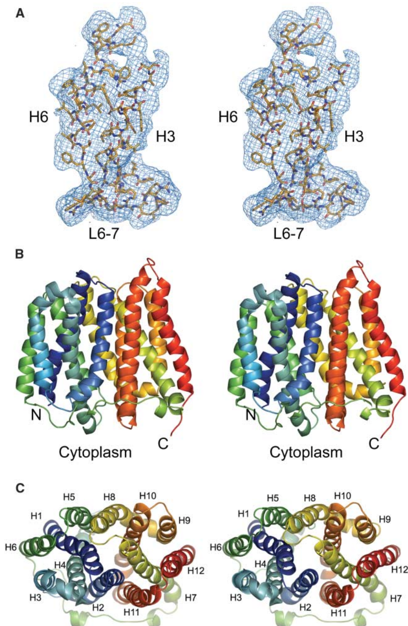
Fig. 1. Stereomages of crystallography and structure of EmrD. (A) A portion of the experimental electron density map is shown for H3, H6, and L6-7. The map is contoured to 1\sigma . (B) Side view of EmrD. The N and C termini are indicated. (C) View of EmrD looking toward the cytoplasm showing the molecular two-fold axis relating the N- and C-terminal halves. Transmembrane helices are indicated. The images were created by PyMol (33).
