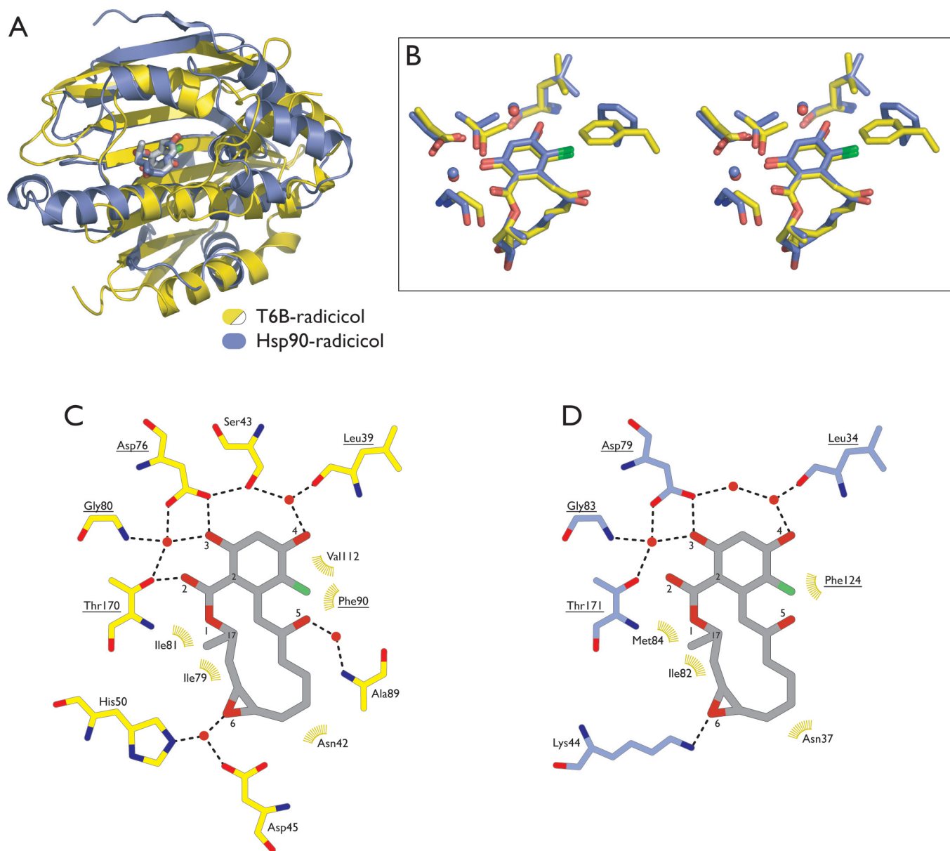
Figure 4. Comparison of radicicol binding to topoVI-B' and Hsp90. (A) Structural overlay of radicicol-bound topoVI-B' (yellow) and Hsp90 (blue) [Ref. (47), PDB code 1BGQ], superposed on the bound radicicol molecule. (B) Stereo view of an overlay between the active sites of topoVI-B' (yellow with red waters) and Hsp90 (blue with blue waters) bound to radicicol, showing a shared constellation of interacting amino acids and liganding water molecules (drug binding residues not shared between the two enzymes are not shown in this panel). (C and D) Detailed views of the interactions of radicicol with topoVI-B' (C) and Hsp90 (D). Drug-liganding amino acids that are conserved between the two proteins are underlined, and oxygen and select carbon atoms of radicicol are numbered.
