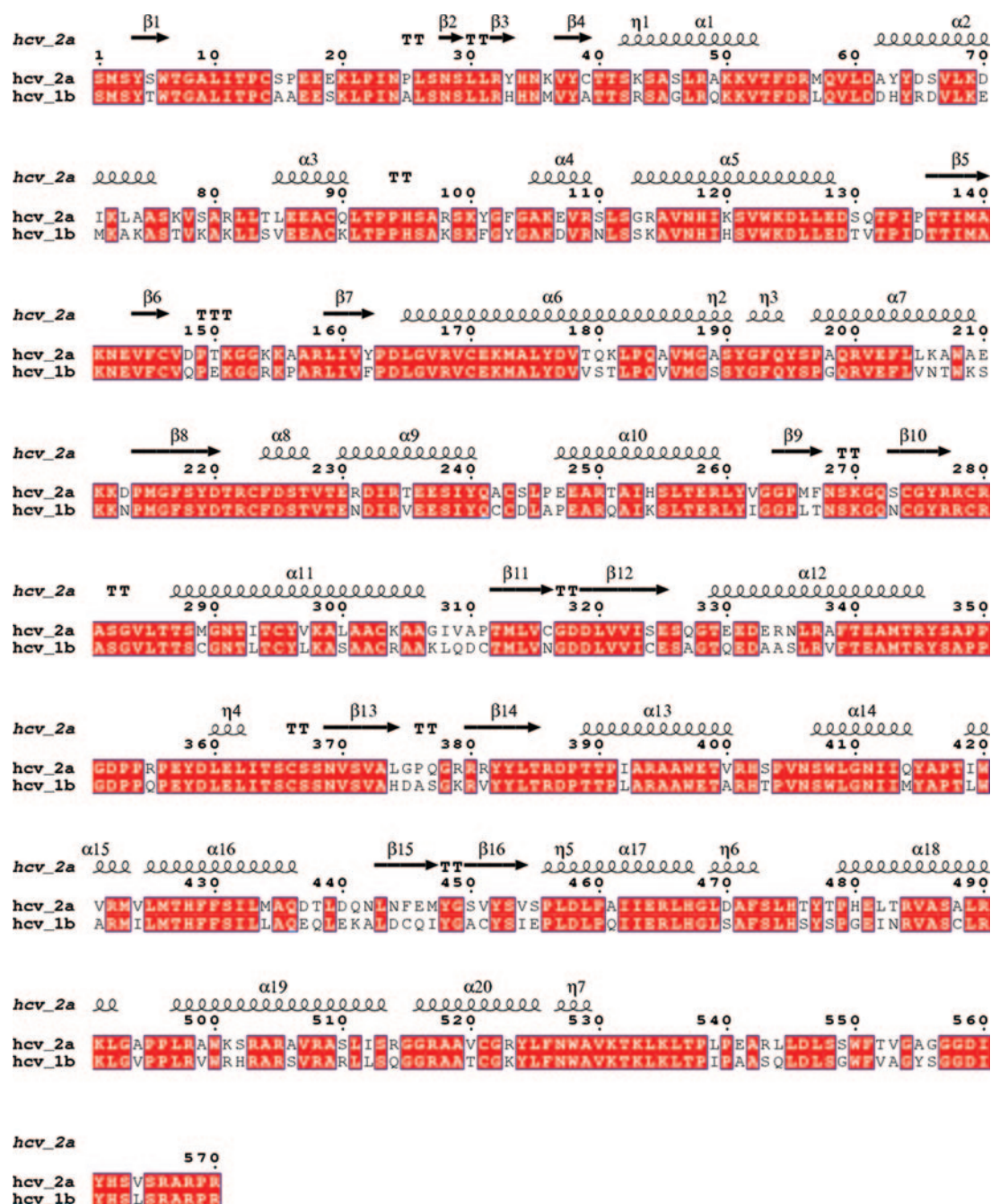
FIG. 5. Comparison of sequences between HCV polymerase genotypes 1b and 2a. Identical residues are shown in the red boxes. Also shown are the secondary structural elements corresponding to the structure of genotype 2a in form II. The figure was generated by the program ESPript (34).
