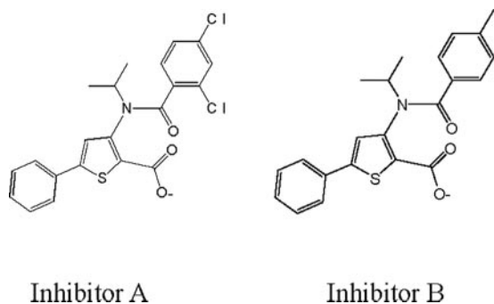
FIG. 1. Chemical structures of non-nucleoside inhibitors A and B.
