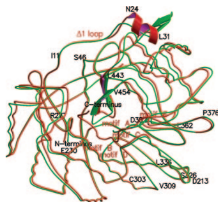
FIG. 3. Stereo view of the overall structure of HCV polymerase genotype 2a in crystal form II. Blue, red, and green colors correspond to the fingers, palm, and thumb domains, respectively. The two loops protruding from the fingers domain are indicated in yellow. Two anti-parallel helices connecting the fingers and palm domains are shown in black. Two active site aspartates are shown by stick representation. The figure was prepared using the program MOLSCRIPT (31).
